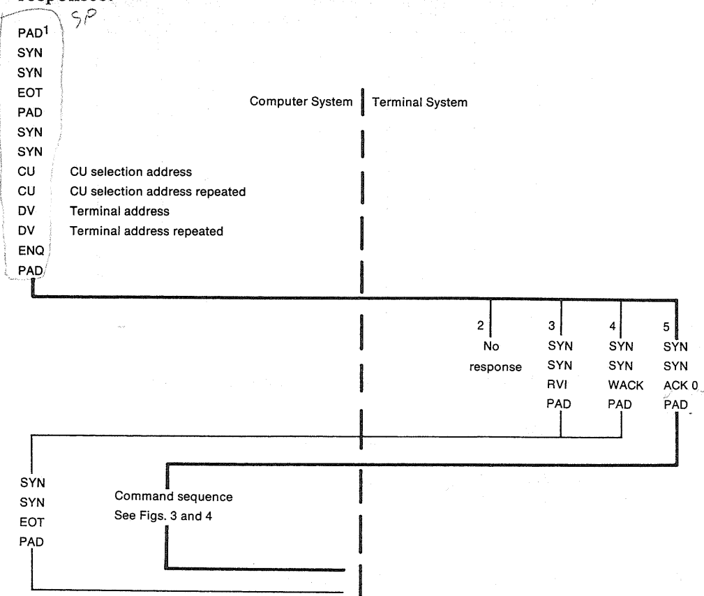
Fig. 2. Selection addressing, sequence diagram
