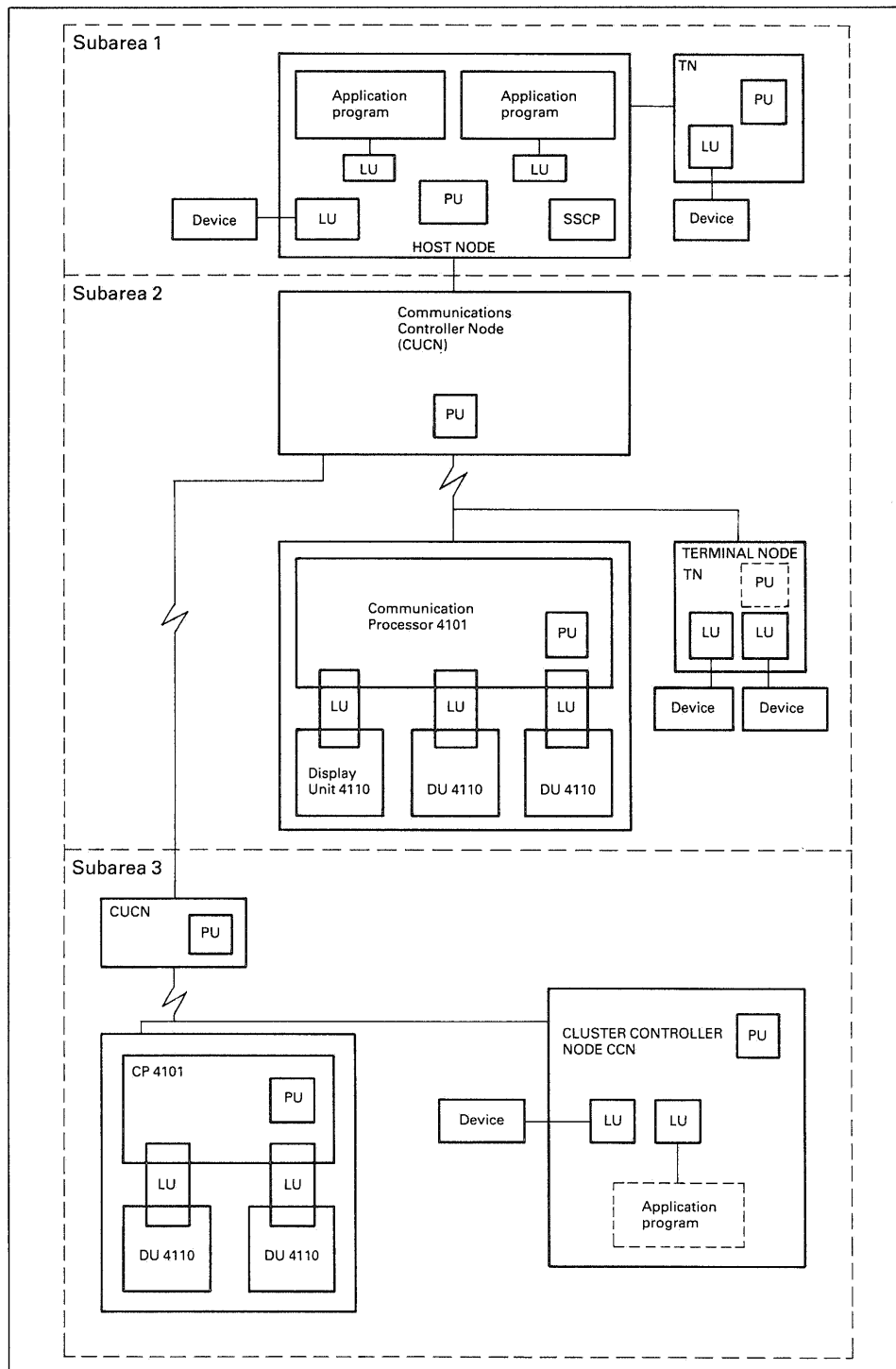
Fig. 2. Relationships between NAUs, nodes and subareas
