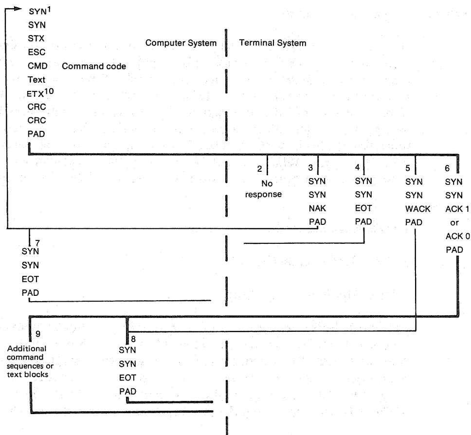
Fig. 3. Write-type and control commands, sequence diagram
