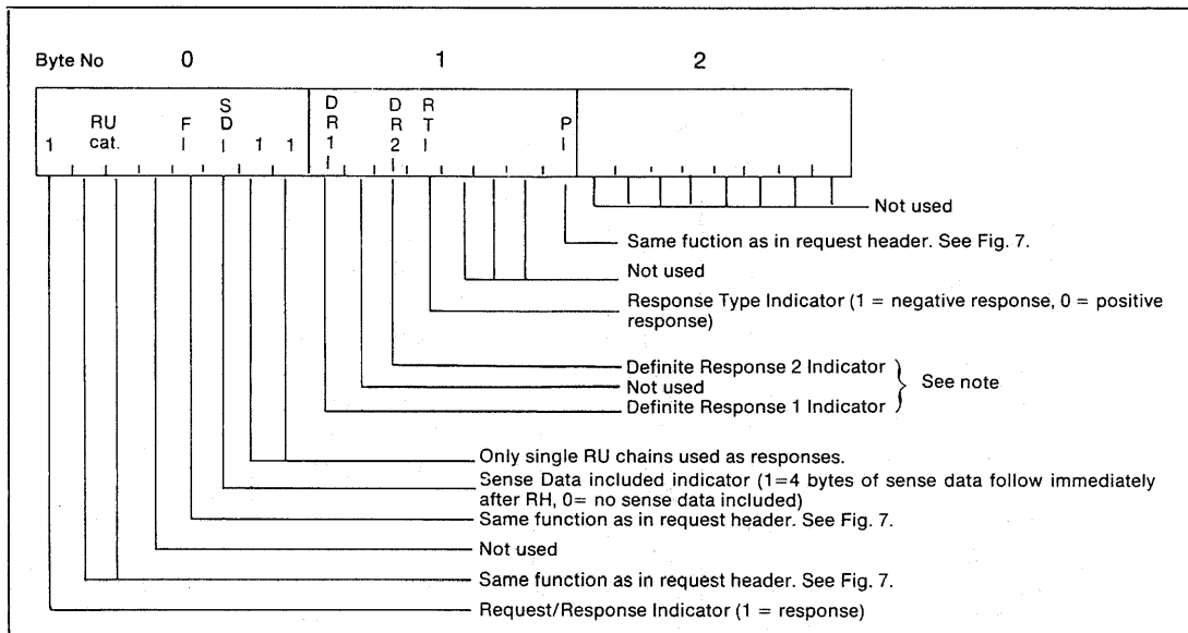
Fig. 8. Response header format
