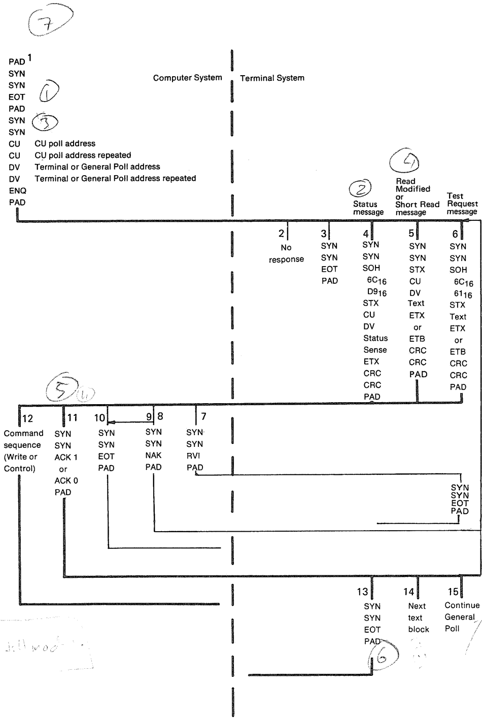
Fig. 1. General and Specific Poll, sequence diagram
