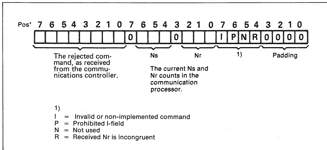
Fig. 13. Information field in the FRMR response frame
