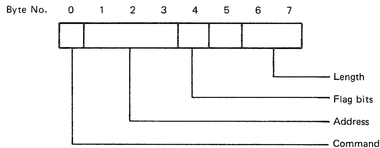
Fig. 1. Channel Command Word format
