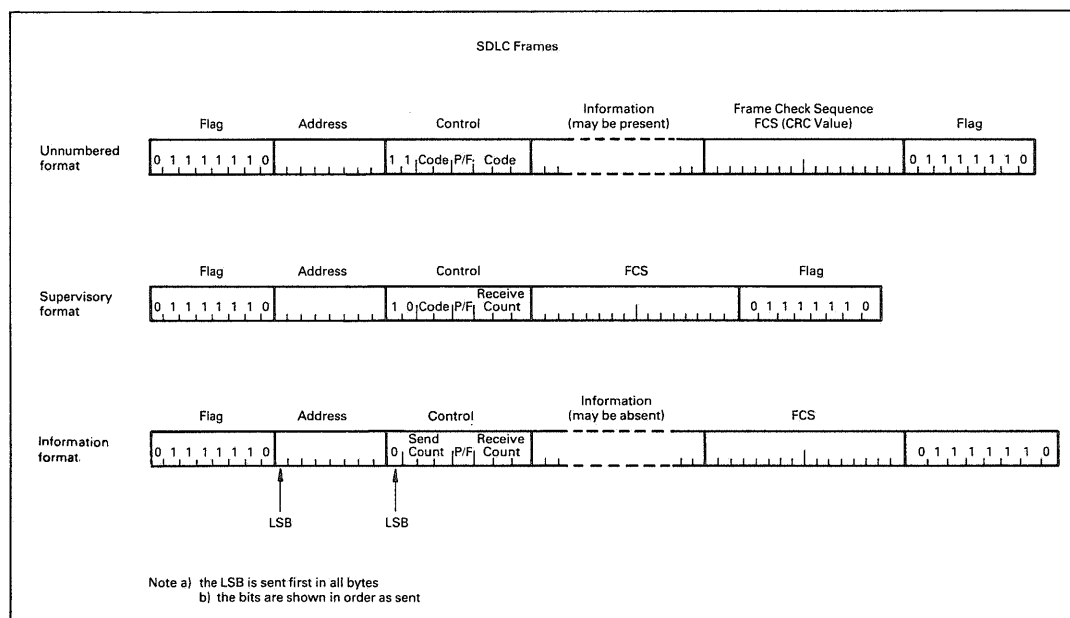
Fig. 12. SDLC frame formats.
