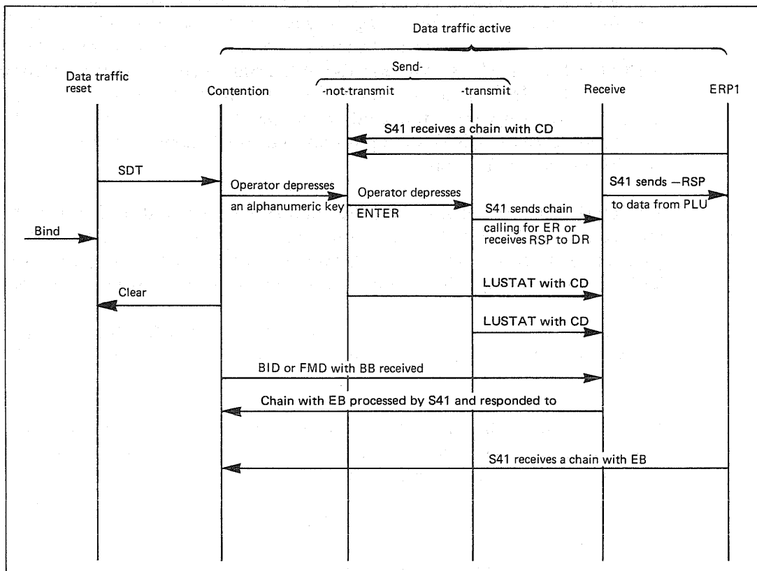
Fig. 9. Session states for LU-LU session
