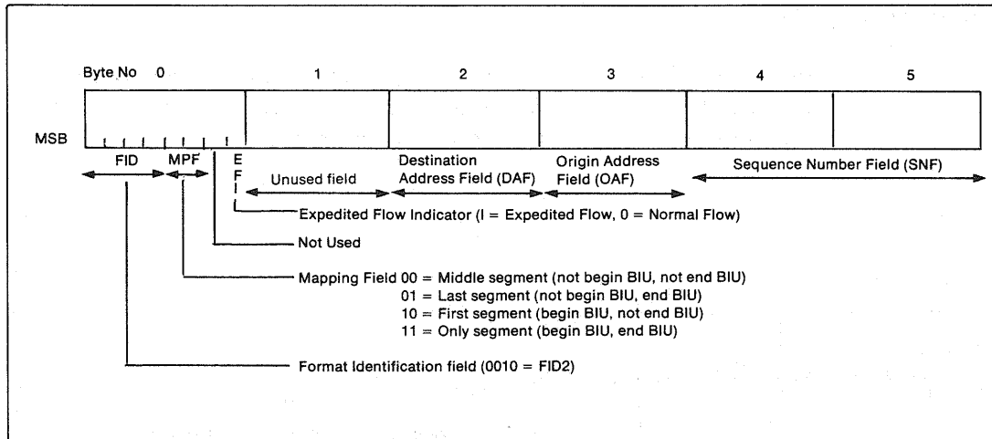
Fig. 6. Transmission header format
