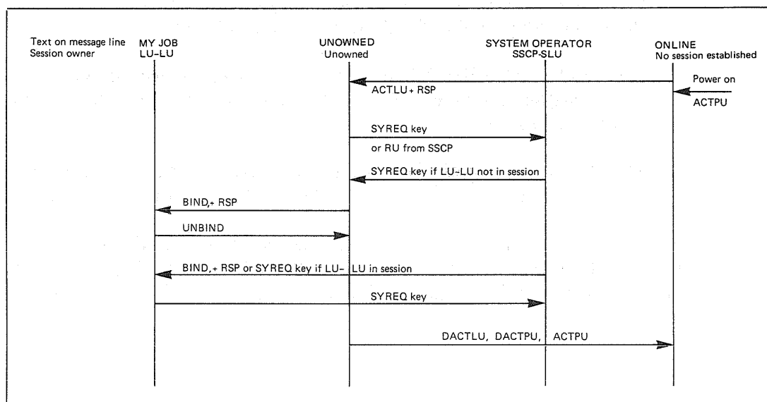
Fig. 11. Session ownership of a Display Unit 4110
