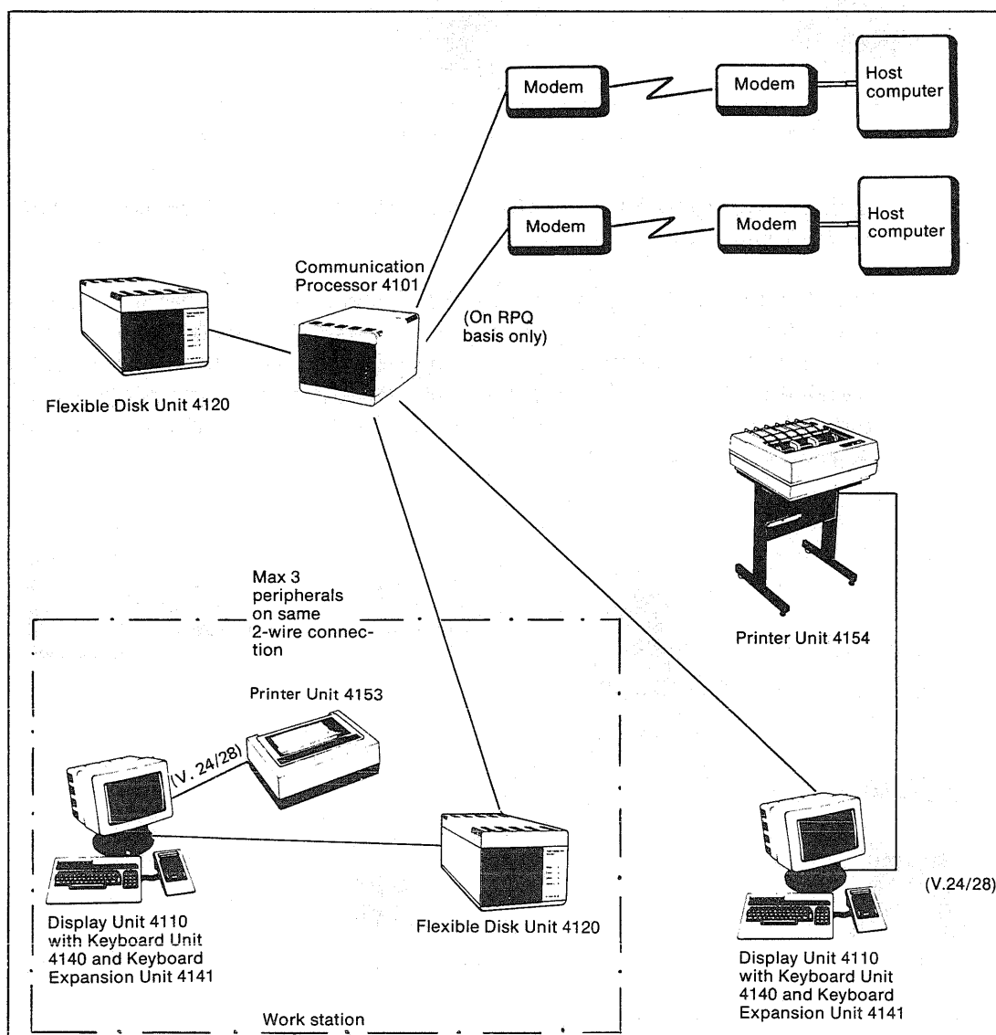
Fig. 1. Cluster configuration connected to remote host computers
