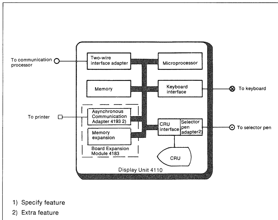
Fig. 8. Block diagram of Display Unit 4110 in cluster configuration
