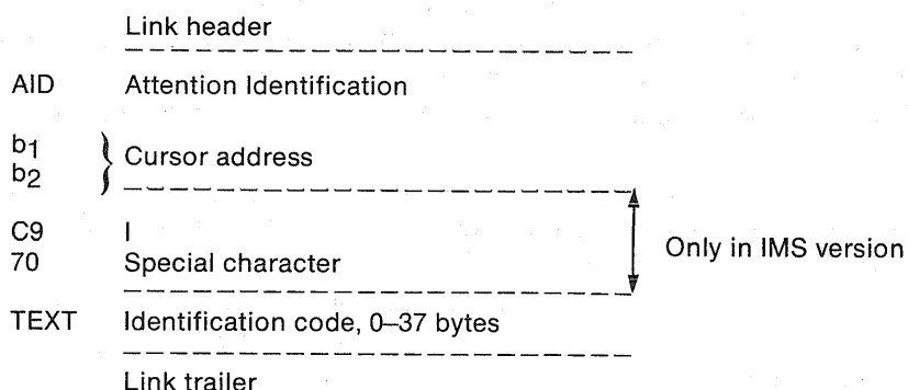
Fig. 3. Message from the terminal issued in connection with a magnetic identification device attention
