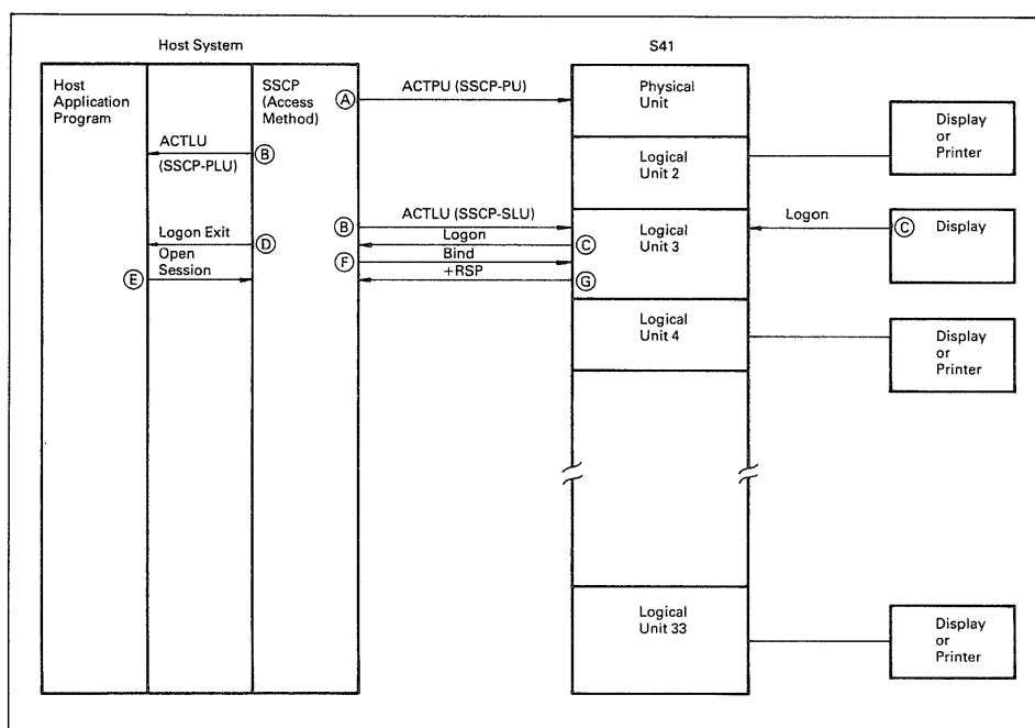
Fig. 5. Establishing a session with an S41
