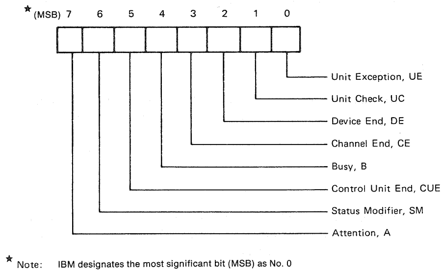
Fig. 2. Status byte bit assignments
