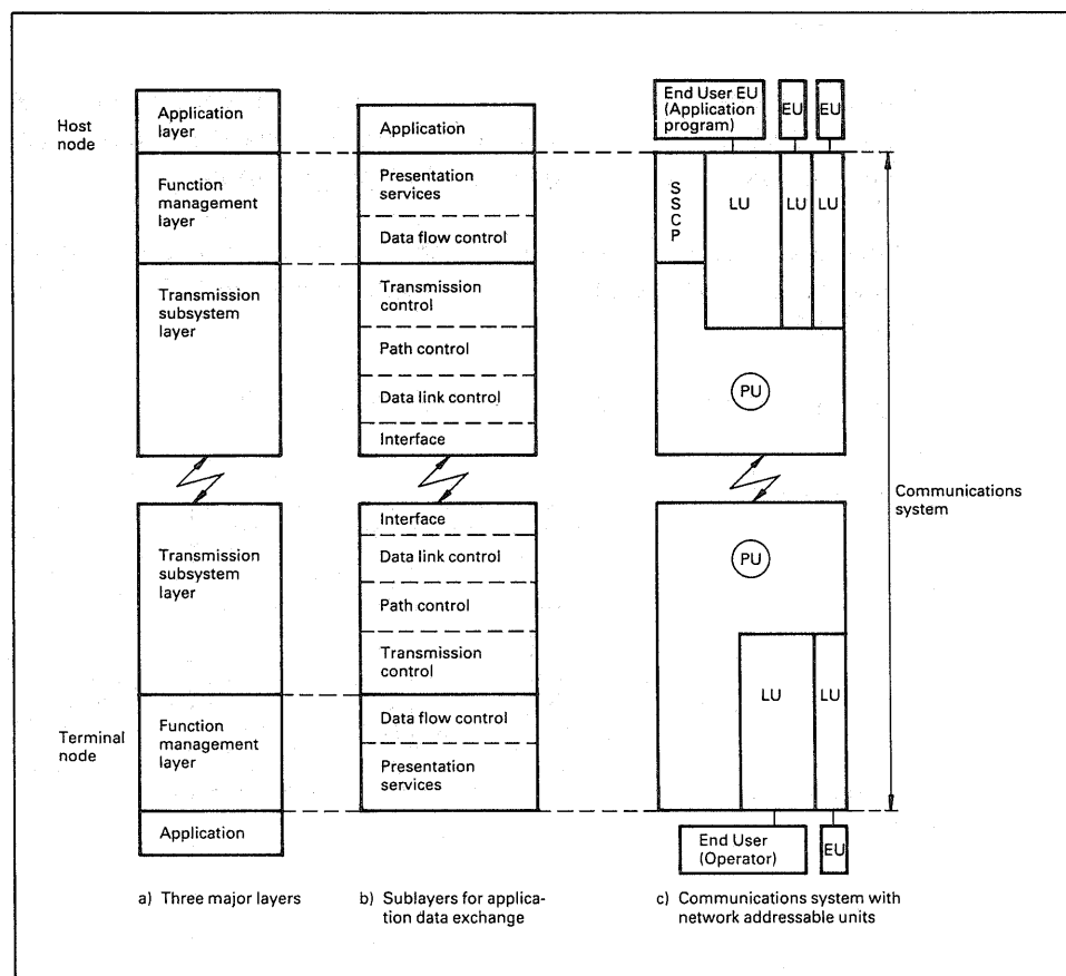
Fig. 1. SNA layering arrangement
