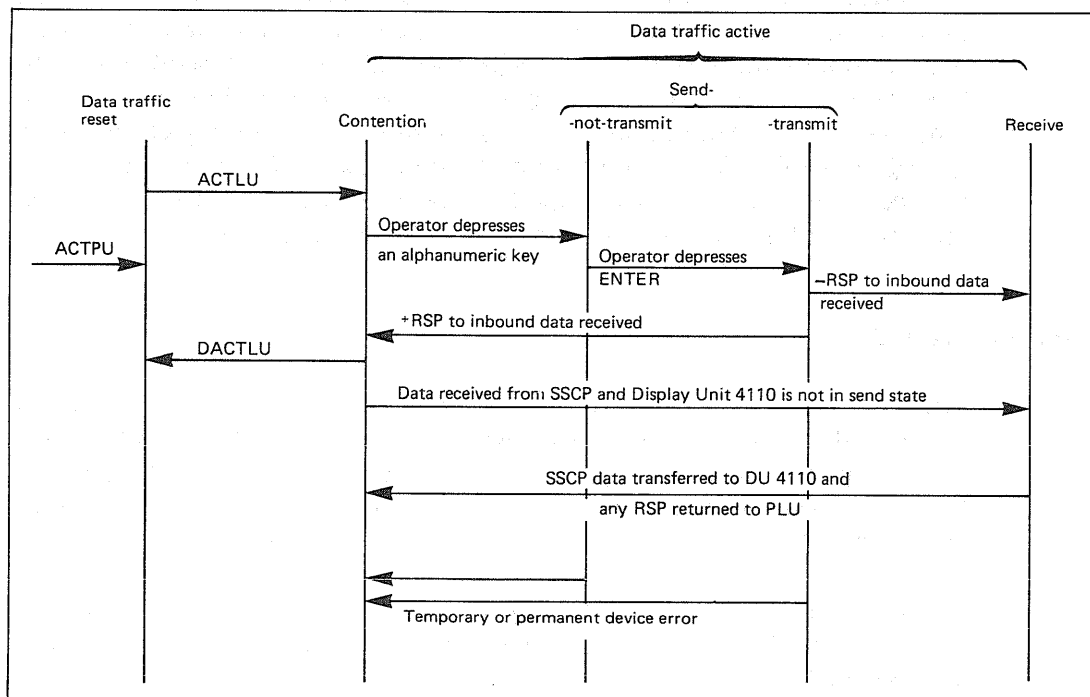
Fig. 10. Session states for SSCP-LU session
