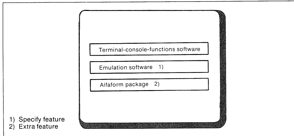
Fig. 16. System software
