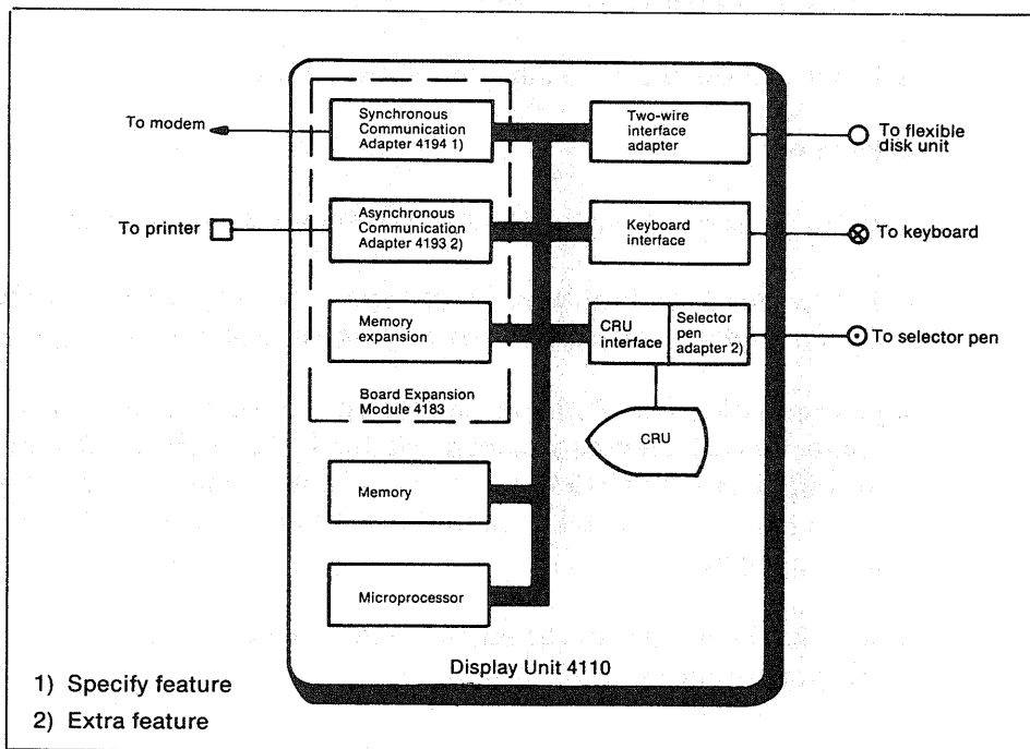
Fig. 9. Block diagram of Display Unit 4110 in single display-unit configuration
