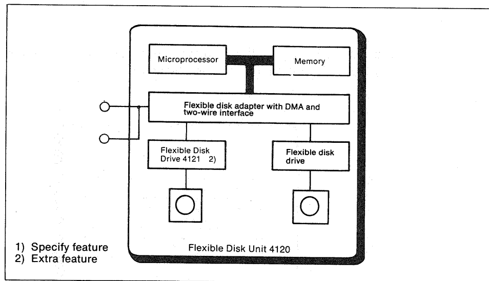
Fig. 15. Block diagram of Flexible Disk Unit 4120
