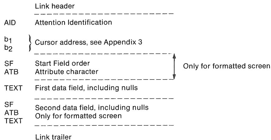
Fig. 1. Message from the terminal issued in connection with a Read Buffer command
