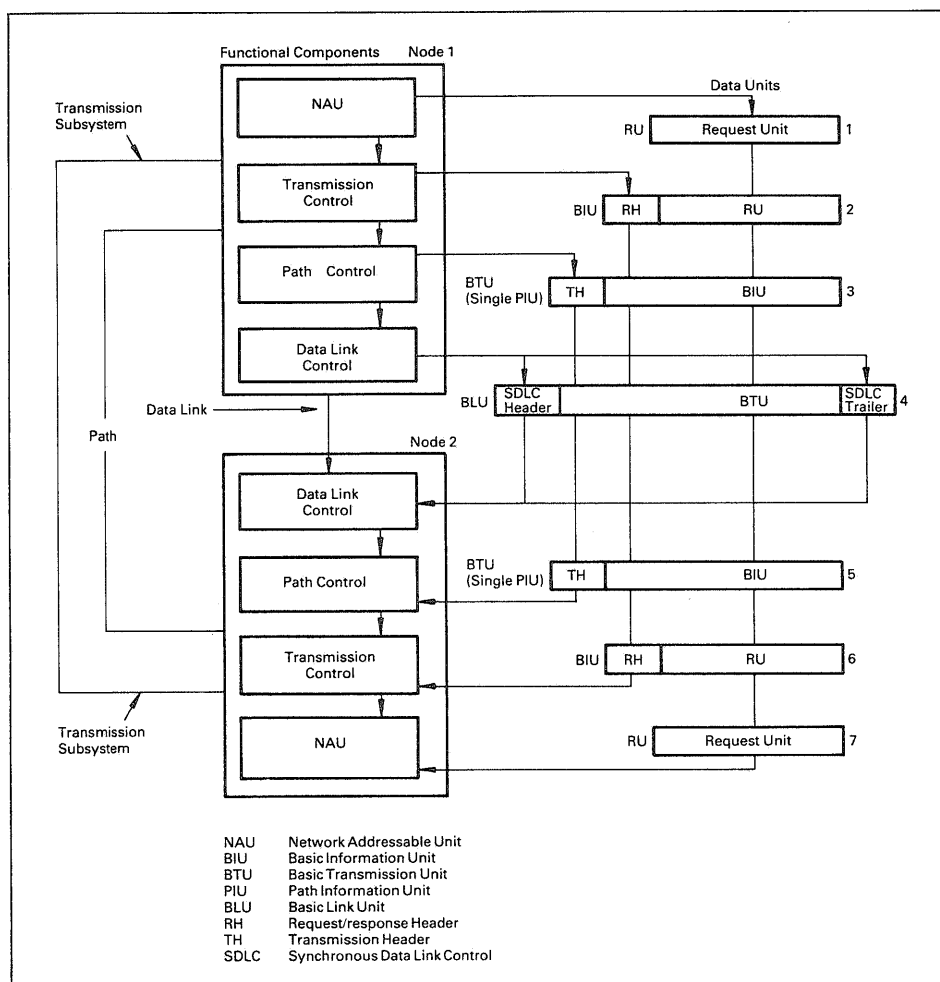
Fig. 3. Diagram showing how headers are added and stripped off
